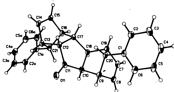
Fig. 1. Dimer ketone with thermal ellipsoids drawn at the 30% probability level. H atoms are represented by spheres of arbitrary size.
